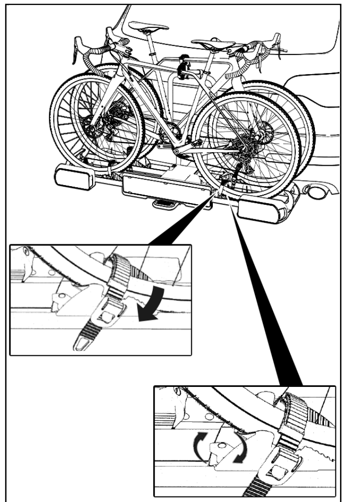
Figure 27: Attaching the rear wheel, second bicycle
